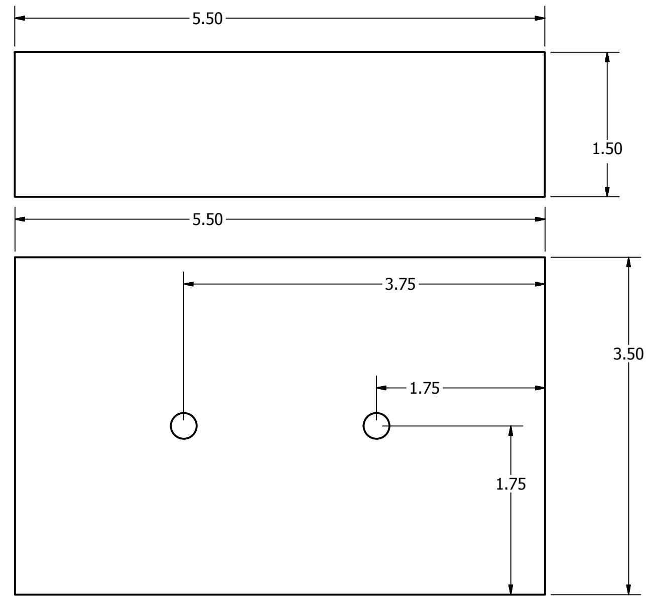
Support block
