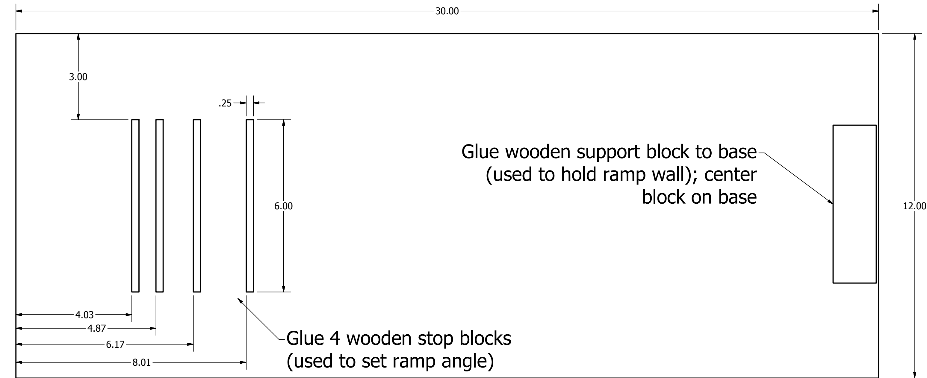
Stand base with glued support and stop blocks (top view)
