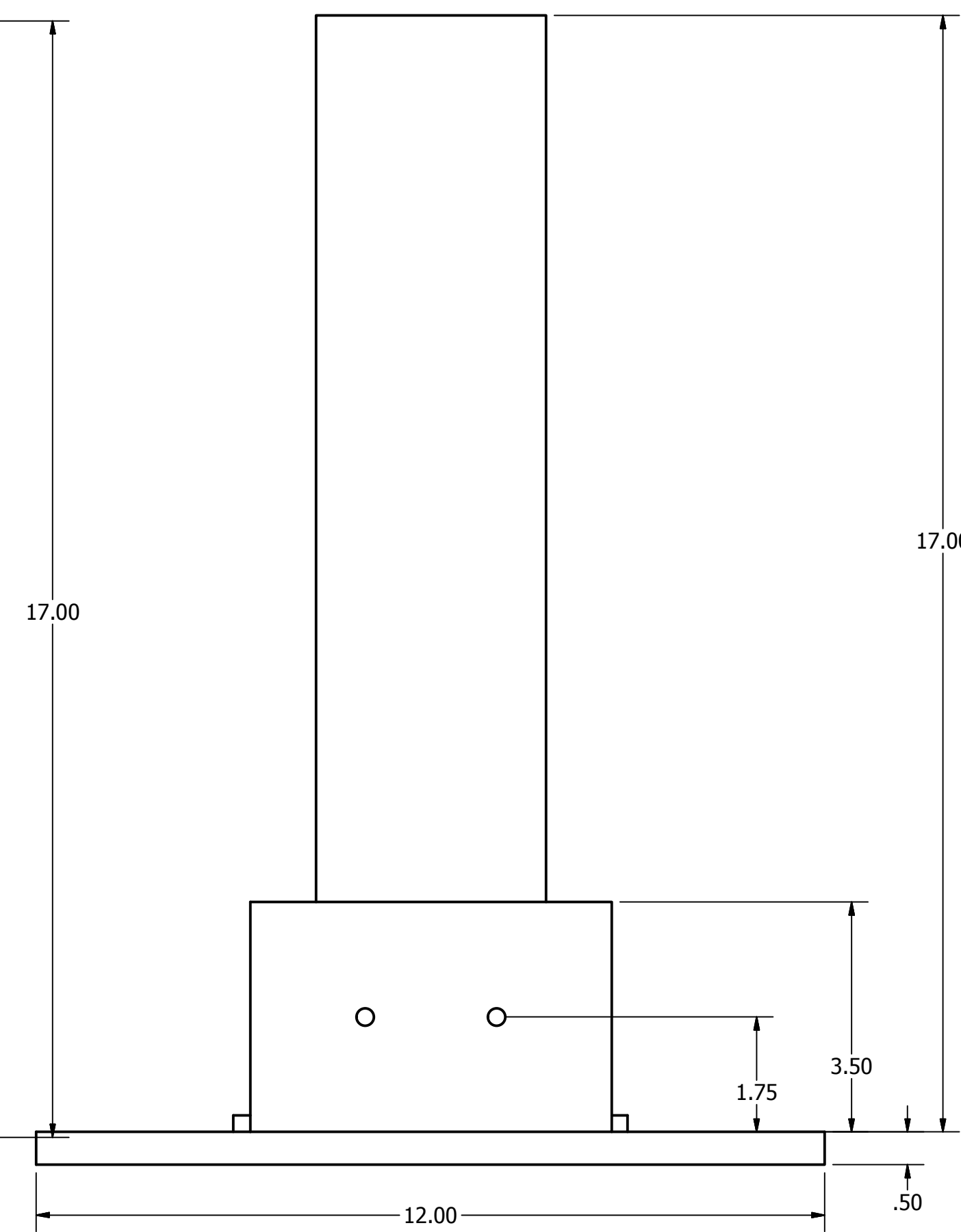
Assembled stand (back view)
