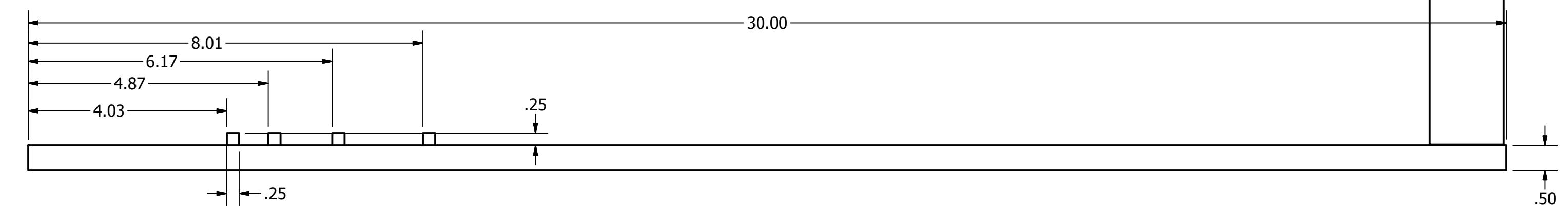
Stand base with glued support and stop blocks (side view)
