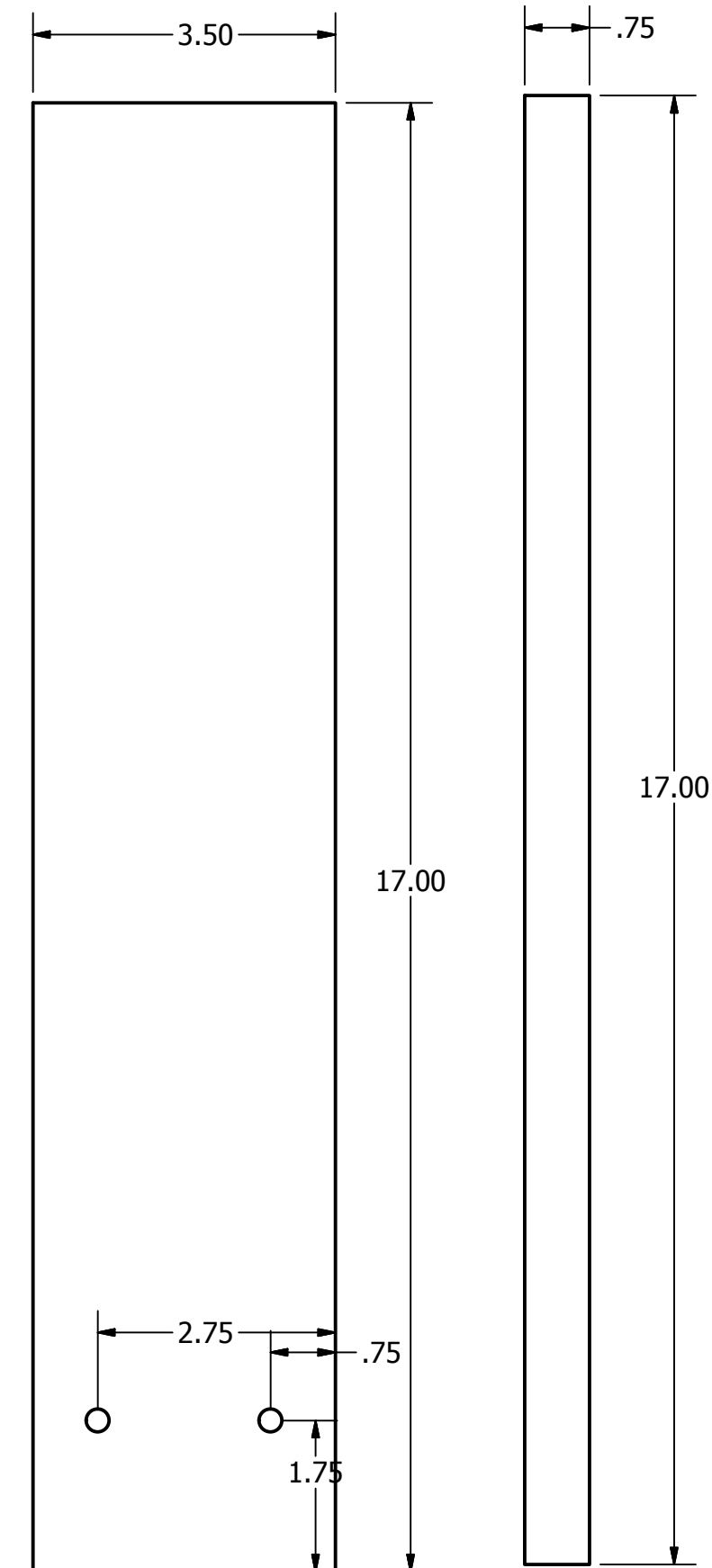
Support wall
