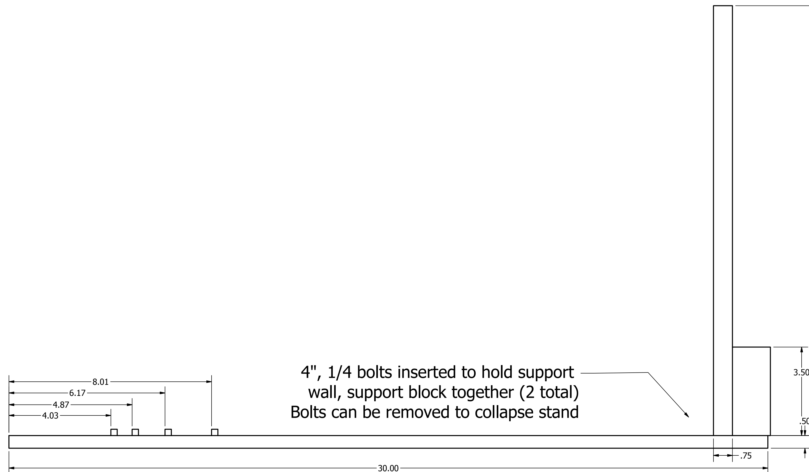
Assembled stand (side view)
