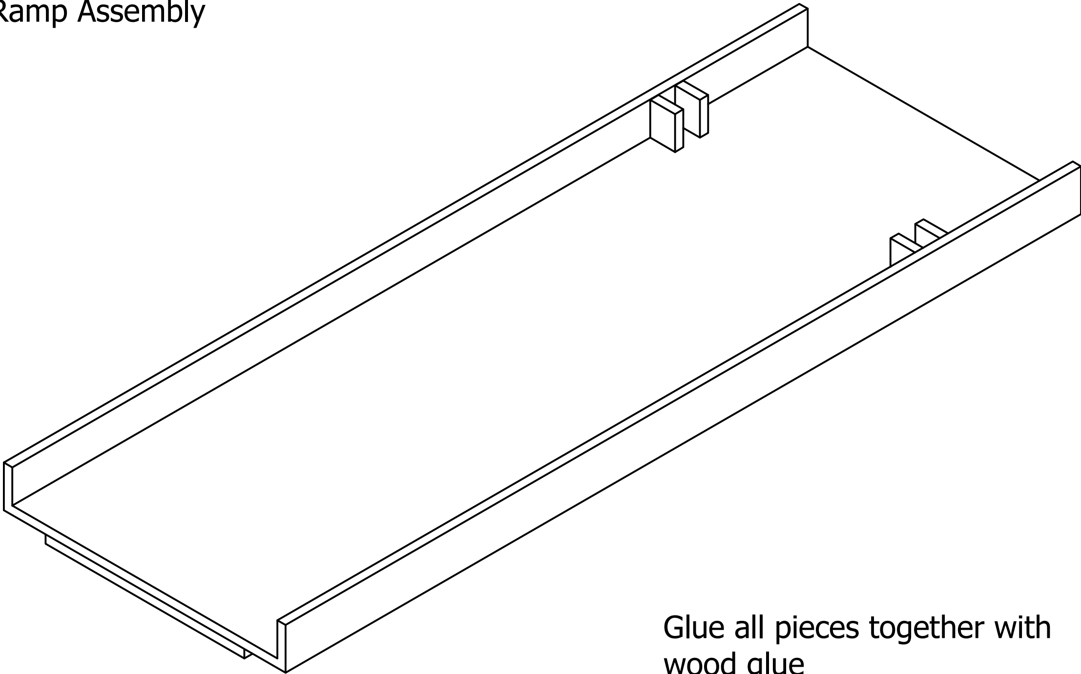
Ramp Assembly
