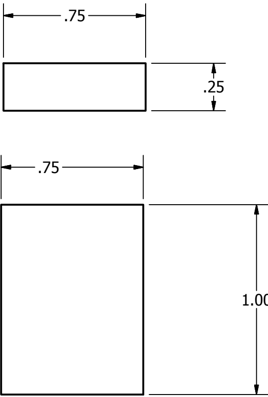
Gate holder: holds wooden gate (need four of these)
