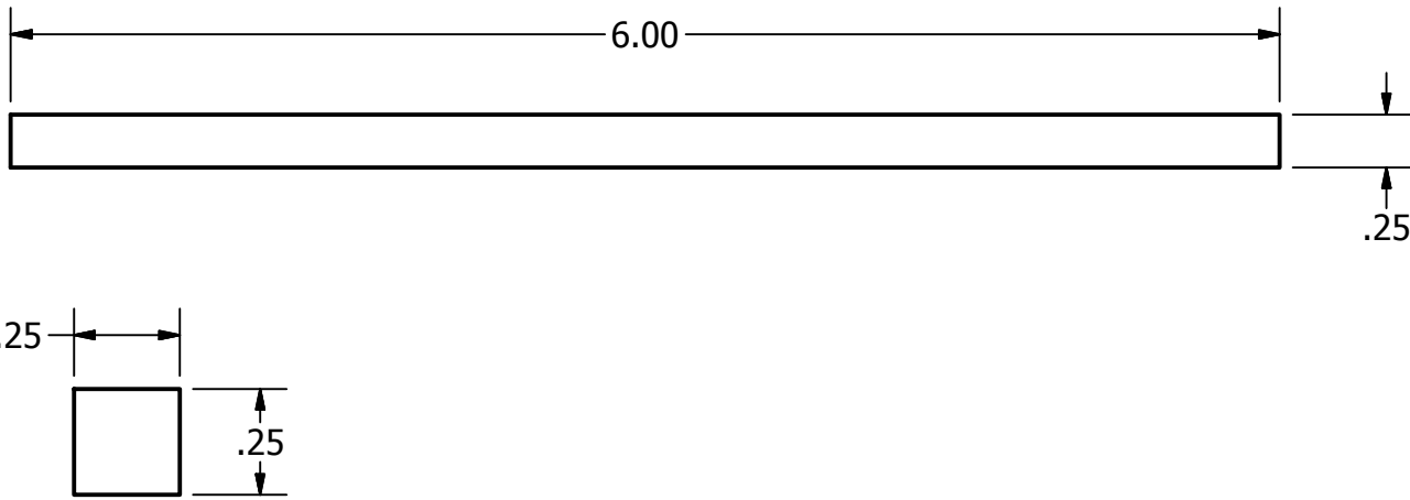
Bottom beam (helps hold ramp against wood base)
